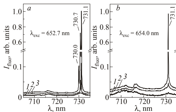
Fig. 4. Fluorescence spectra and stimulated emission from H 2 TBP molecules in nitrogen matrix at 8 K ( \lambda_{\text{exc}} = 652.7 (a) and 654.0 (b) nm, P_{\text{laser}} \approx 10 (1), 30 (2) and 100 (3) mW).
