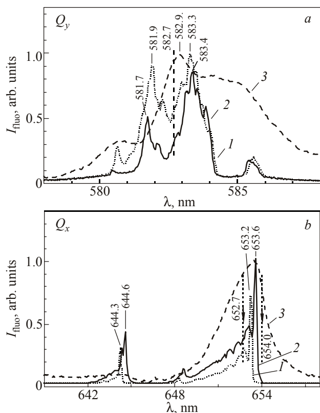
Fig. 3. Comparison of the excitation spectra of the stimulated emission (1 and 2) and the absorption spectrum (3) from H 2 TBP molecules in nitrogen matrix at 8 K for S_2 \leftarrow S_0 ( \lambda_{\text{obs}} = 730.7 (1) and 731.0 (2) nm) (a) and S_1 \leftarrow S_0 ( \lambda_{\text{obs}} = 730.7 (1) and 731.1 (2) nm) (b).
