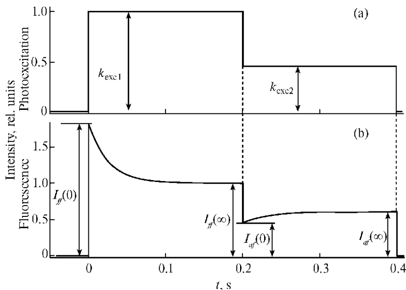
Fig. 1. (a) The shape of the two-step photoexcitation pulse; (b) schematic representation of FF and AF kinetics for a hypothetical metalloporphyrin molecule ( k_{exc1} = 18.5 \text{ s}^{-1} , k_{exc2} = 8.5 \text{ s}^{-1} , p = 22 \text{ s}^{-1} , f = 10^7 \text{ s}^{-1} , and k_{ST} = 5 \times 10^8 \text{ s}^{-1} ).
