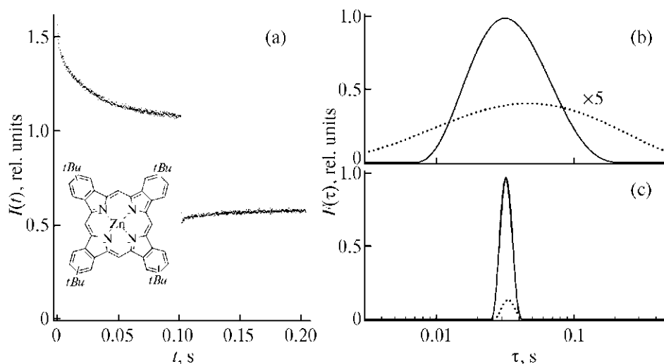
Fig. 3. (a) Experimental curves of FF and AF kinetics of Zn (tBu) 4 -TBP in PVB at 77 K. Calculated spectral density of characteristic times F(\tau) for (b) noisy and (c) smoothed with the Daubechies wavelet filter experimental curves of the FF (solid lines) and AF (dashed lines) kinetics.
