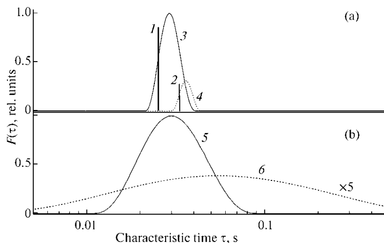
Fig. 2. Spectral density of characteristic times F(\tau) of simulated (1, 3, 5) FF and (2, 4, 6) AF kinetics for a typical metalloporphyrin ( f = 1 \times 10^7 \text{ s}^{-1} , k_{ST} = 5 \times 10^8 \text{ s}^{-1} , p = 22 \text{ s}^{-1} , k_{exc1} = 18.5 \text{ s}^{-1} , and k_{exc2} = 8.5 \text{ s}^{-1} ). (a) Calculations in the approximation of (1, 2) one- and (3, 4) three-dimensional models in the absence of the noise. (b) Calculations in the approximation of (5, 6) a three-dimensional model at a maximum amplitude of the noise equal to \pm 0.033I(0) .
