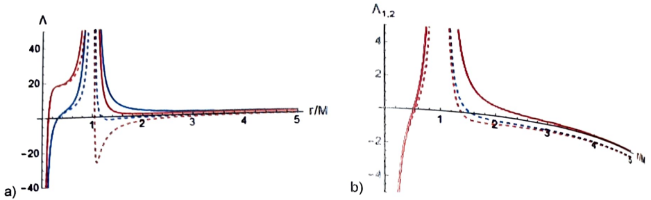
Figure 1. Typical dependencies of the second invariant eigenvalues on the radial coordinate x = \frac{r}{M} for the Schwarzschild spacetime
